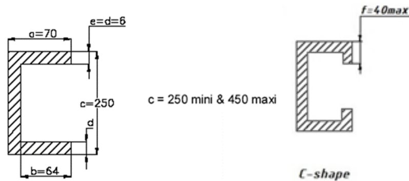
Dessin / Drawing 287-5
