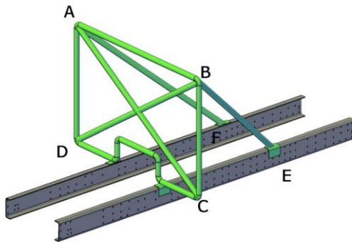
Dessin / Drawing 287-3
