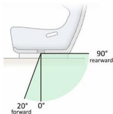
Dessin / Drawing 253-61
