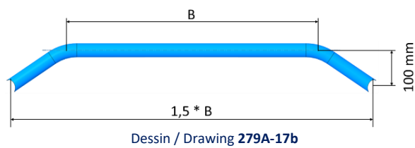
Dessin / Drawing 279A-17
