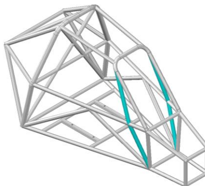
Dessin / Drawing 279A-11
