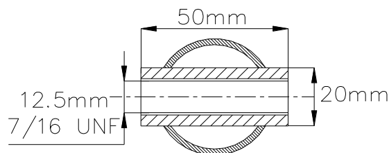
Dessin / Drawing 253-67
