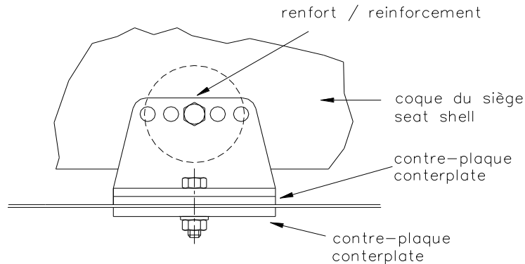
Dessin / Drawing 253-65
