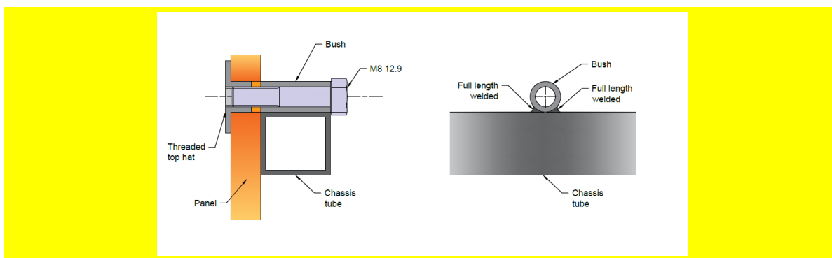
Figure 3. Method for fixing the panel to the chassis (for square tubes only)
