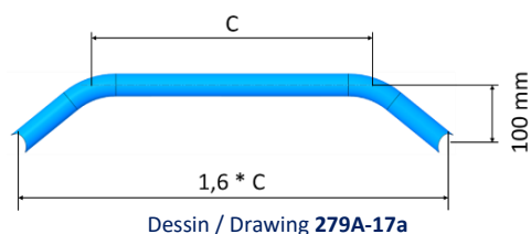
Dessin / Drawing 279A-17a
