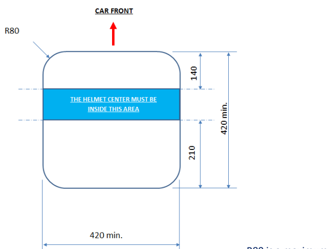
Dessin / Drawing 257A-3
